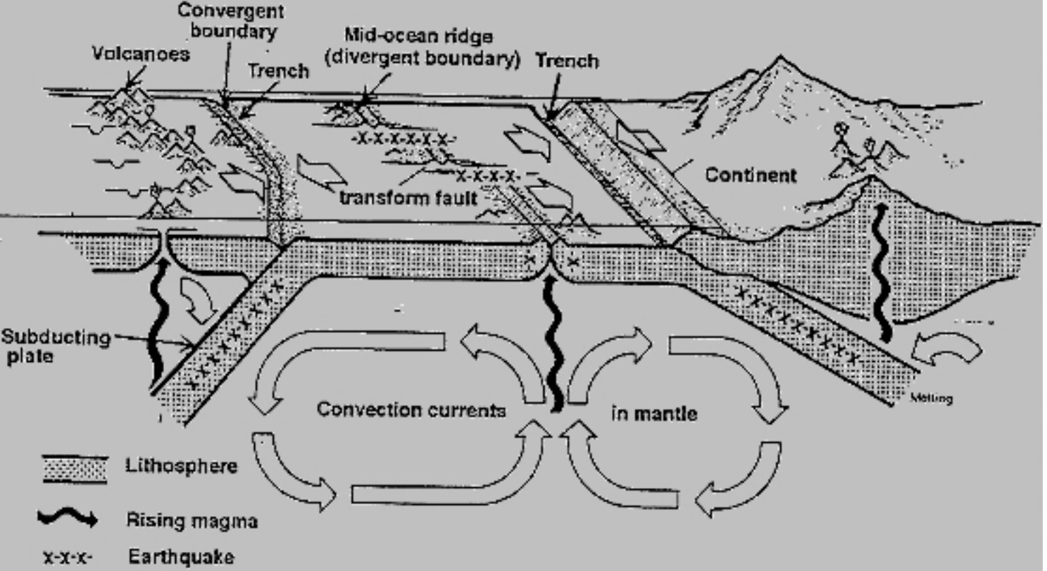
Figure 2. Sea-floor spreading. Modified from NSTA/FEMA (1988).
